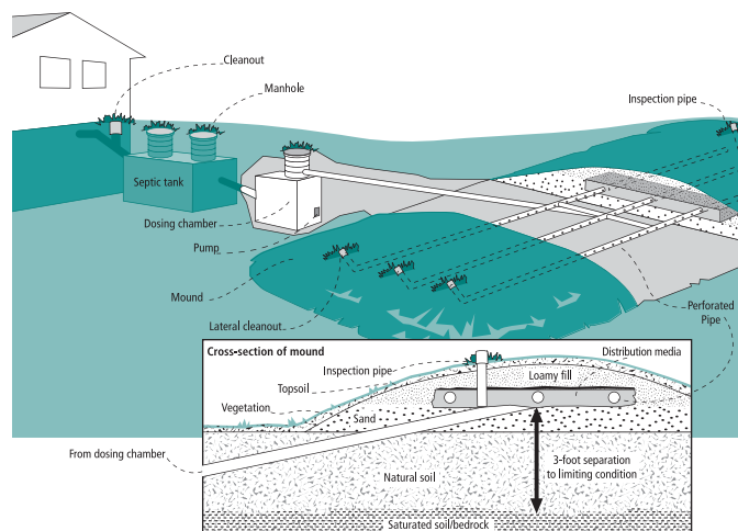
Figure 1. Cross section of a mound system.
